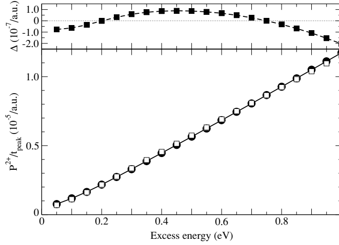
Figure 2. Scaled probability P^{2+}/t_{\text{peak}} for photo-double ionization of He ( 1s^2\ ^1S ) as a function of the excess energy: \square s -wave counterlinear model data, \bullet convolved Wannier power law (11) with P_{0.75\text{ eV}}^{2+} = 3.8387 \times 10^{-4} . The upper panel shows the difference \Delta ( \blacksquare ) between the two data sets.
